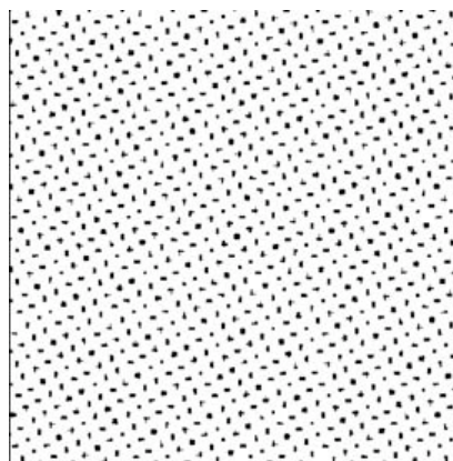
Figure 2 A typical mesh blocking between a 380 mesh and a 150 lpi screen at 20% dot at 30° to the mesh. Although this is a calculated image, it looks very close to the real thing.
