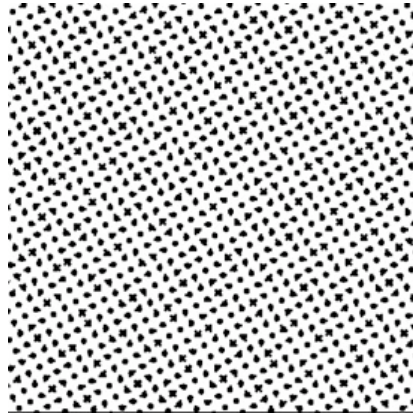
Figure 3 The same mesh and screen as Figure 2 but this time a high Rz stencil leads to the classic starry dot created by leaks through the poor gasket.
