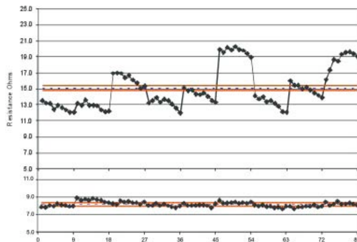
The high-Rz, low-EOM emulsion stencil (top) gives large variations in resistance over the 81 variants of squeegee pressure/angle/orientation compared to the low-Rz, low-EOM capillary film (below).
