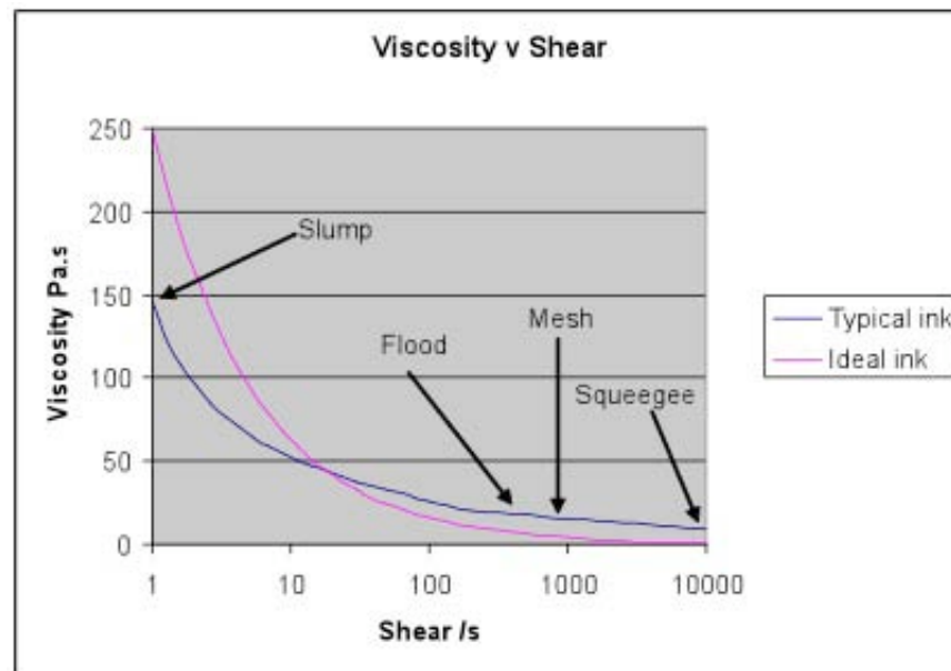
Viscosity v Shear for a typical ink and an ideal ink
