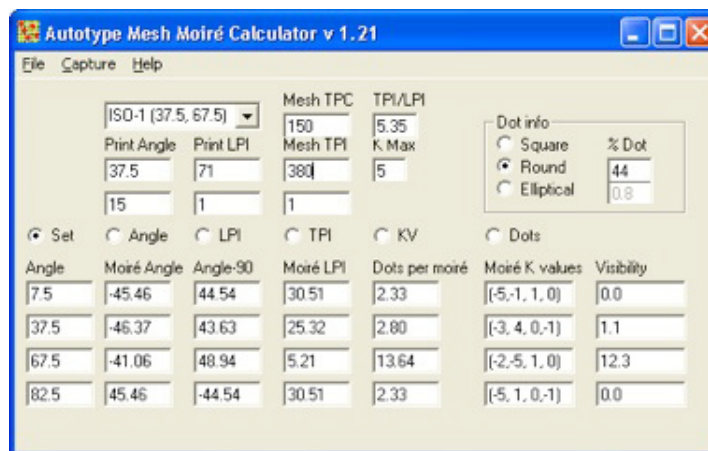
Figure 6a. A change to a 380 (150) mesh lets you print the 37.5° with no problem, but the 67.5° would be a disaster.
