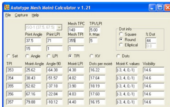
Figure 6 The moiré now changes by a large amount (e.g. the angle changes from 25.62 to 79.88°) for the same small change in mesh count.
