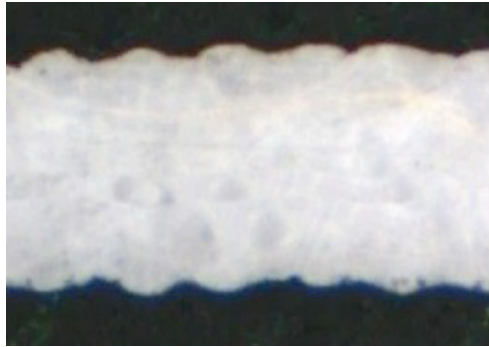
The classic result of a high Rz stencil – positive sawtoothing
