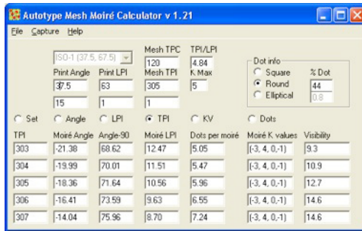
Figure 5 The moiré does not change all that much (e.g. the angle changes from -21.38 to -14.04°) when the thread count changes by a modest amount.
