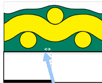
Undercutting caused by positive in poor contact with the stencil
