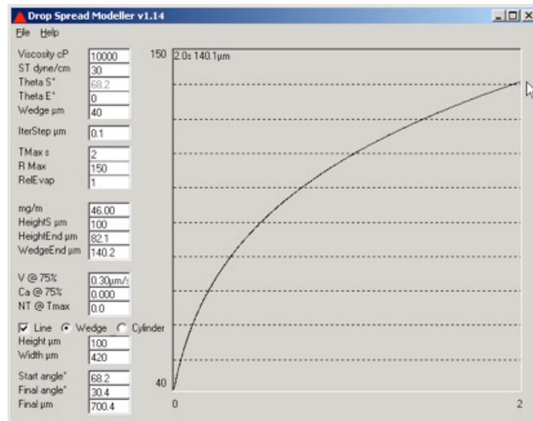
The Drop Spread software models the 100μm high, 500μm wide line
