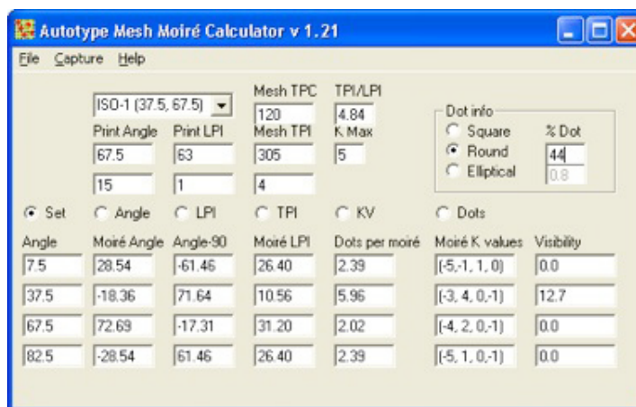
Figure 4 Calculating the mesh moiré possibilities for a 63 lpi print with a 305 mesh (25/120)
