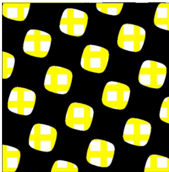
Figure 7. You might think that the threads in the middle of the hole in the stencil will block the flow of ink, giving very serious thread eclipse. But given adequate squeegee pressure, a low viscosity ink and a thin stencil, ink can flow around the thread and print a full dot. When the thread is at the edge of a hole, it would block half the thread diameter, unless you have the right stencil/ink combination. This is the same 2.54 mesh to stencil ratio as used in calculating the mesh moiré in Figure 2.
