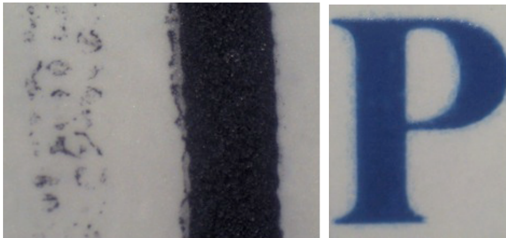
Slur: in both these prints we had a slack mesh and excessive squeegee pressure
